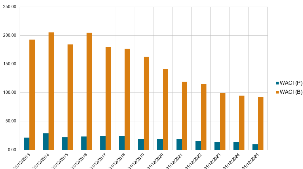
Figure 7: Weighted Average Carbon Intensities (WACI) Trend Chart (tCO2e/$m) for the period 2013-2025
