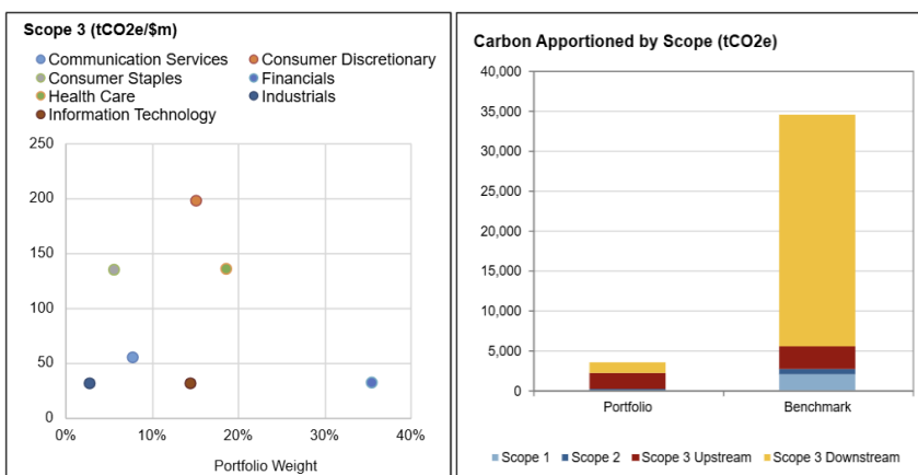
Figure 7: Emissions by Scope
