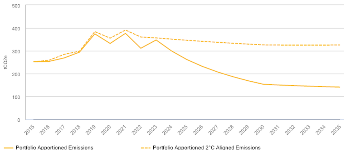
Figure 8: 2°C Alignment Portfolio Transition Pathways
